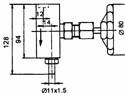
drain valve type 17/500 (sleeve G 3/8"):
