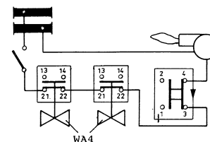
Magnetic switch M130K in level controller/limiter
